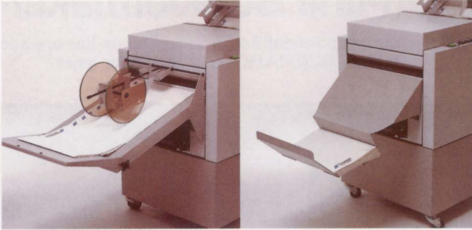
Two different delivery systems. Belt Stacker (left) for larger volumes and Delivery Tray (right). Optional
